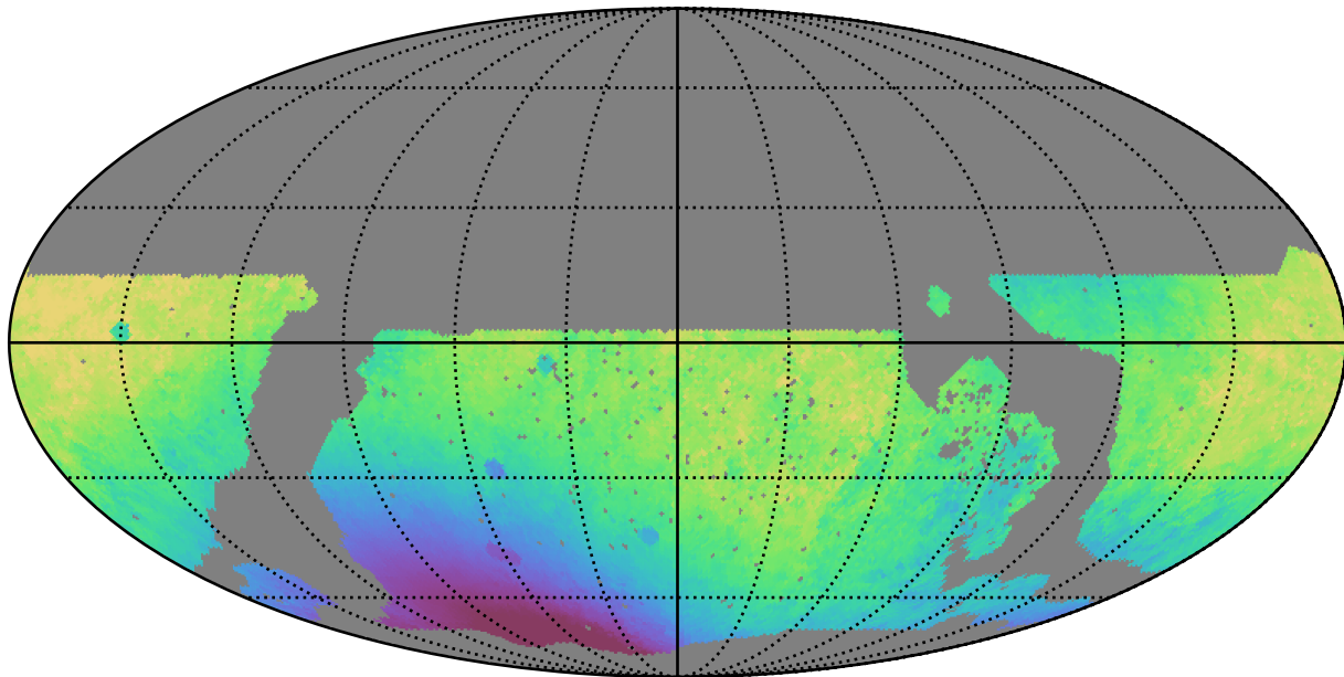
noroll_v3.4_10yrs WFD r band: Median solarElong
