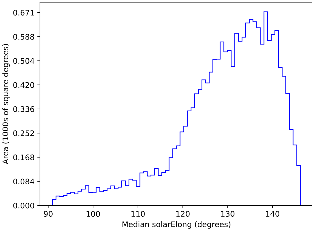
noroll_v3.4_10yrs WFD r band: Median solarElong
