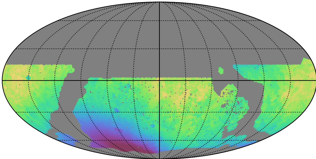
noroll_v3.4_10yrs WFD i band: Median solarElong
