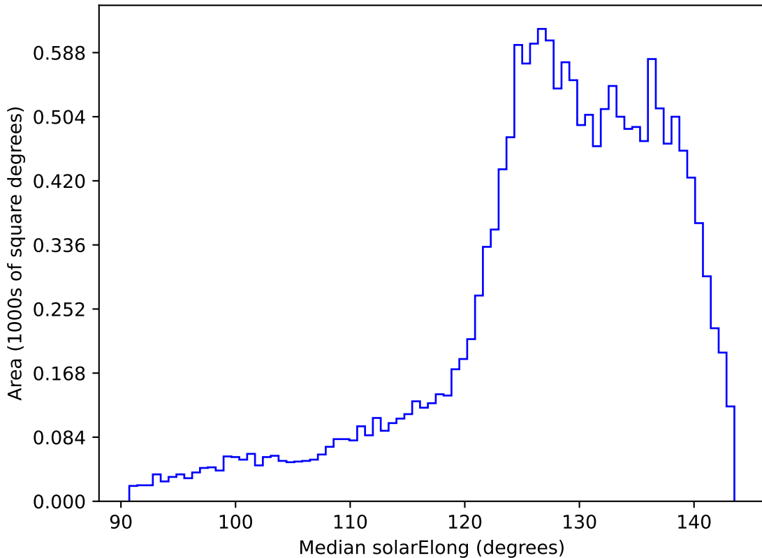
noroll_v3.4_10yrs WFD i band: Median solarElong
