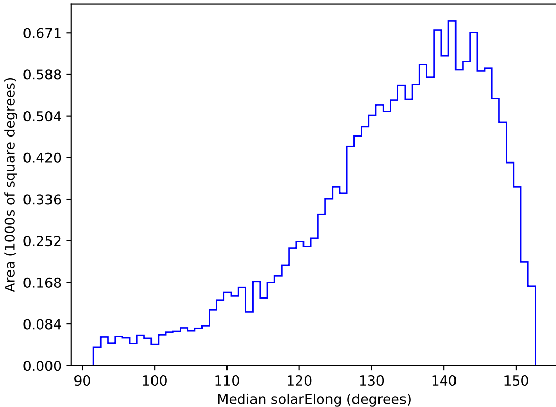
noroll_v3.4_10yrs WFD g band: Median solarElong
