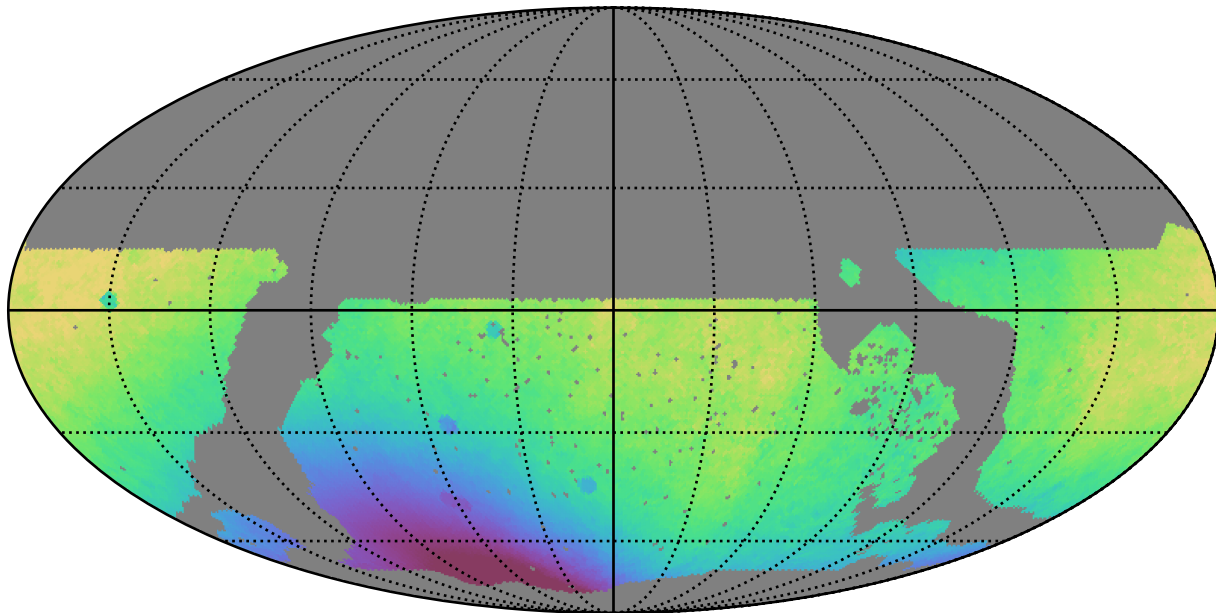
noroll_v3.4_10yrs WFD all bands: Median solarElong
