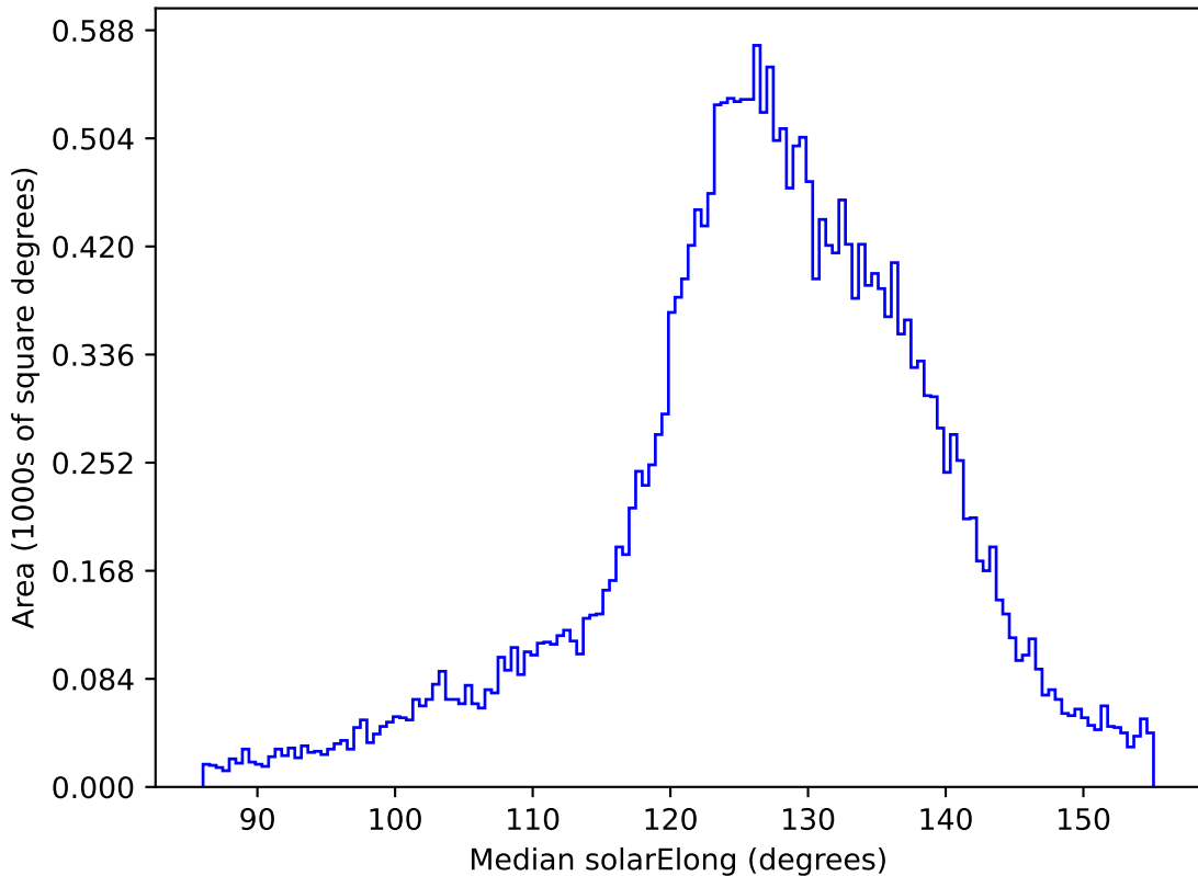
noroll_v3.4_10yrs All sky z band: Median solarElong
