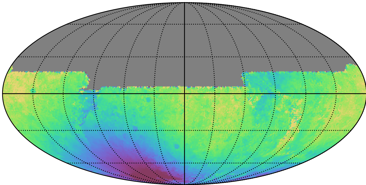
noroll_v3.4_10yrs All sky y band: Median solarElong
