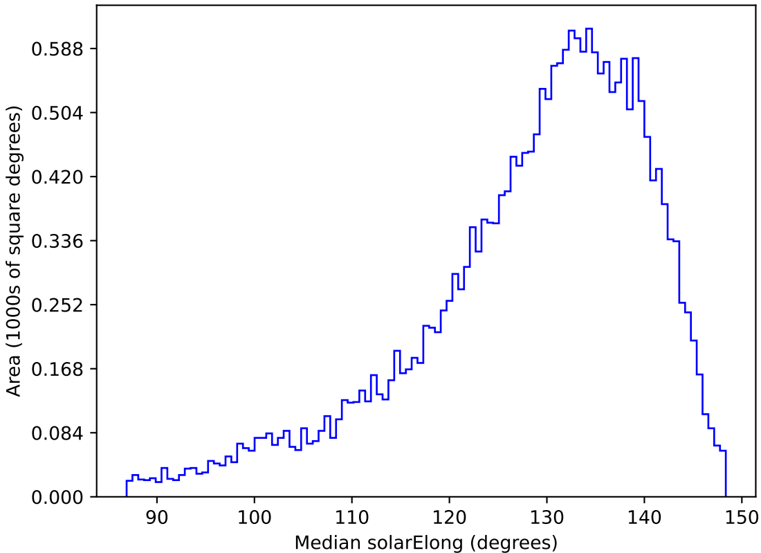
noroll_v3.4_10yrs All sky y band: Median solarElong
