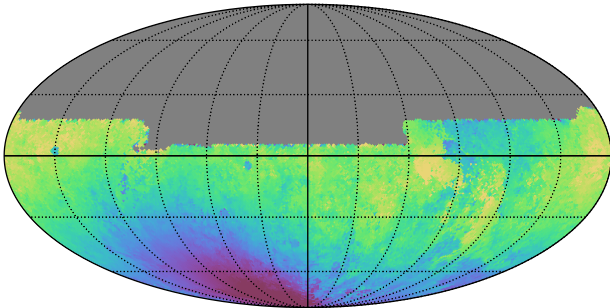
noroll_v3.4_10yrs All sky u band: Median solarElong
