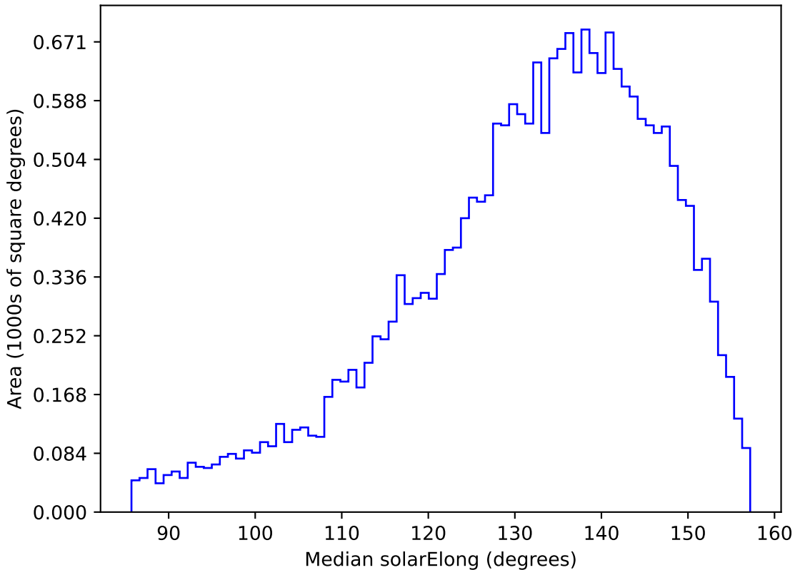
noroll_v3.4_10yrs All sky u band: Median solarElong
