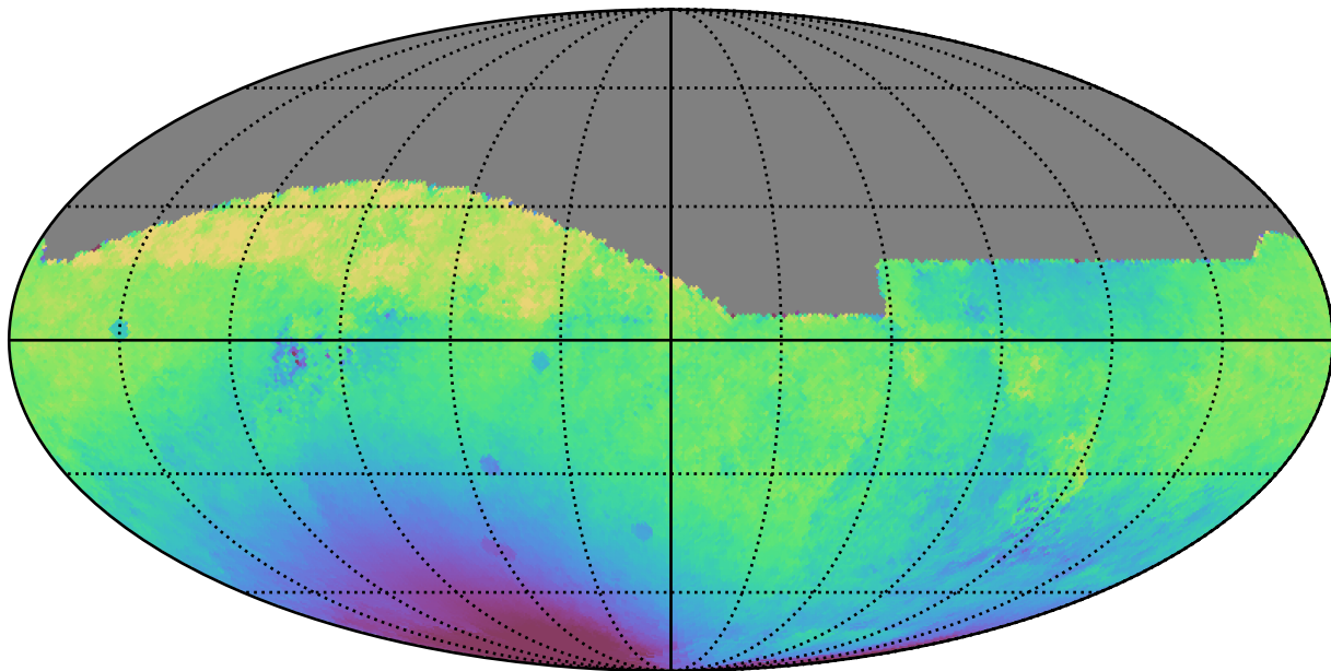
noroll_v3.4_10yrs All sky r band: Median solarElong
