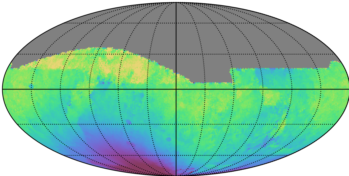
noroll_v3.4_10yrs All sky i band: Median solarElong
