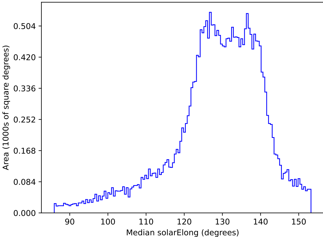
noroll_v3.4_10yrs All sky i band: Median solarElong
