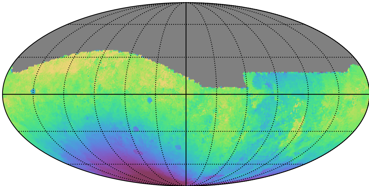
noroll_v3.4_10yrs All sky g band: Median solarElong
