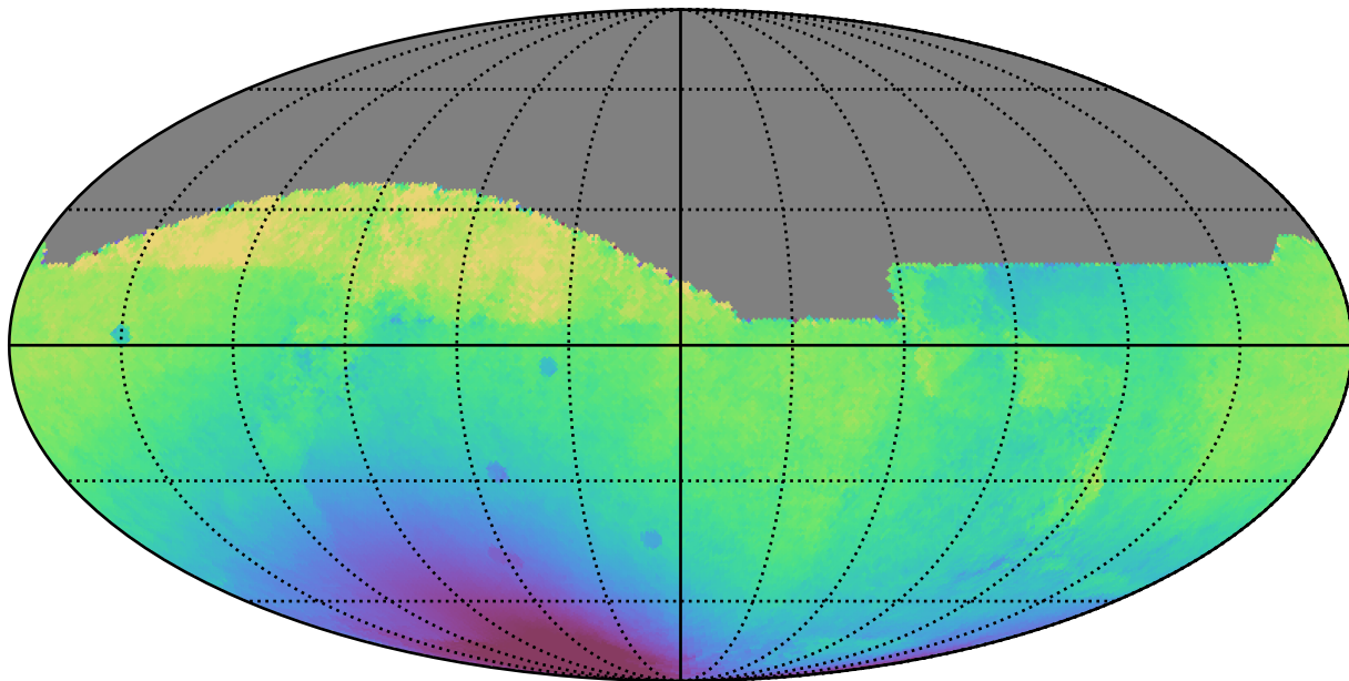
noroll_v3.4_10yrs All sky all bands: Median solarElong
