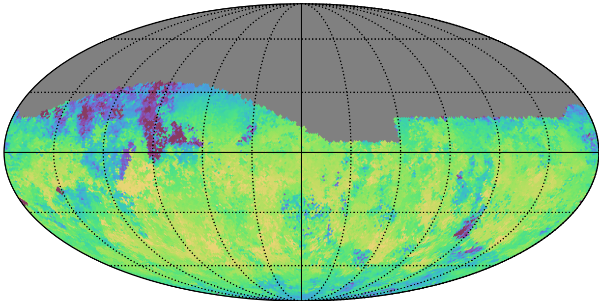
noroll_v3.4_10yrs Yr 1 z band: Median skyBrightness
