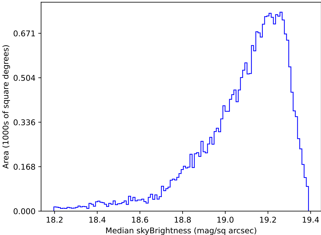
noroll_v3.4_10yrs Yr 1 z band: Median skyBrightness
