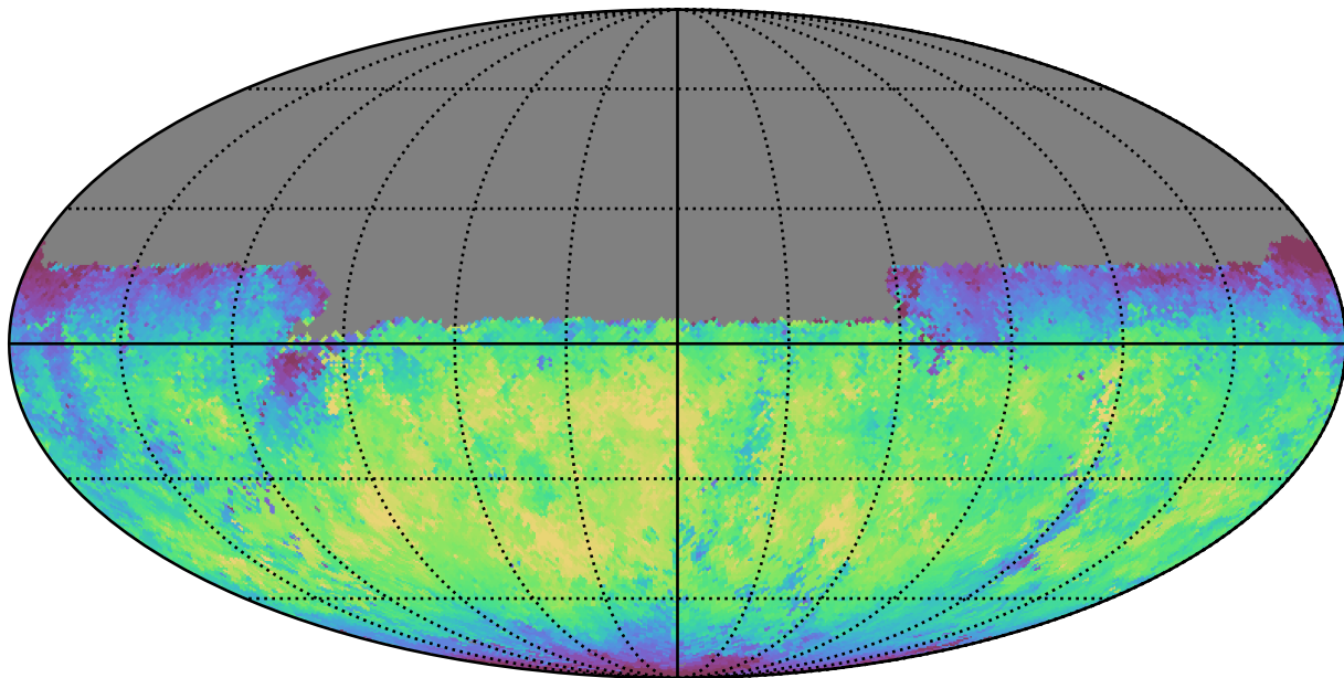
noroll_v3.4_10yrs Yr 1 y band: Median skyBrightness
