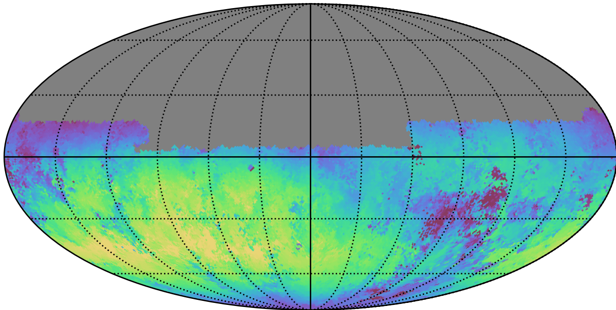
noroll_v3.4_10yrs Yr 1 u band: Median skyBrightness
