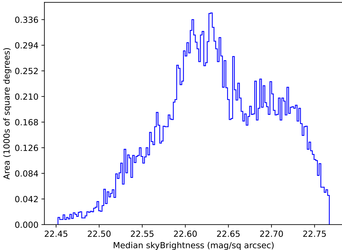
noroll_v3.4_10yrs Yr 1 u band: Median skyBrightness
