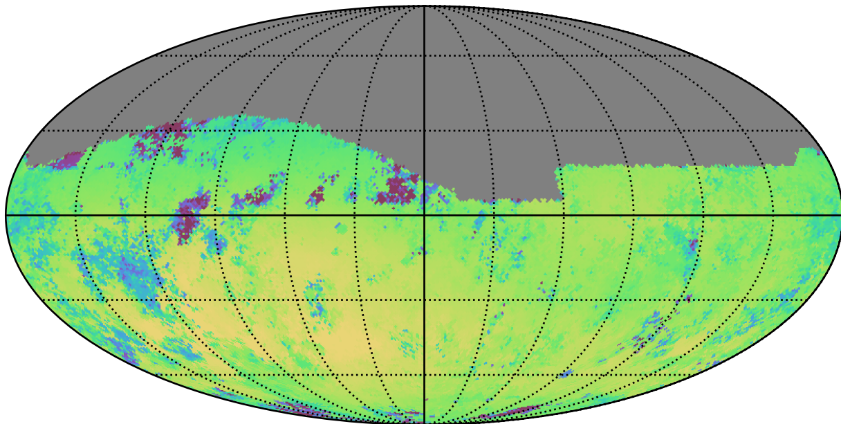
noroll_v3.4_10yrs Yr 1 r band: Median skyBrightness
