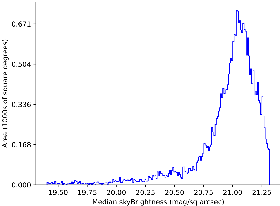
noroll_v3.4_10yrs Yr 1 r band: Median skyBrightness
