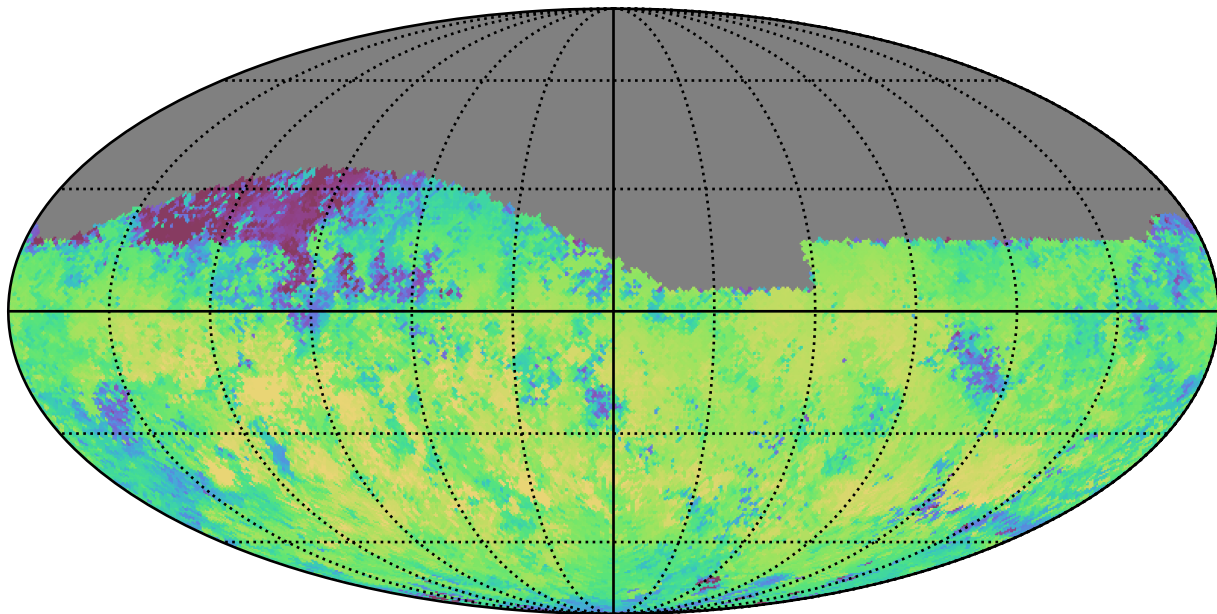
noroll_v3.4_10yrs Yr 1 i band: Median skyBrightness
