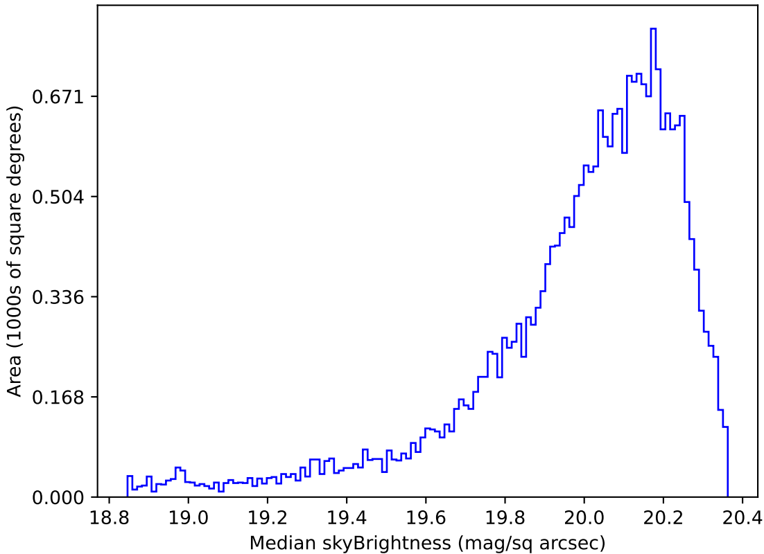
noroll_v3.4_10yrs Yr 1 i band: Median skyBrightness
