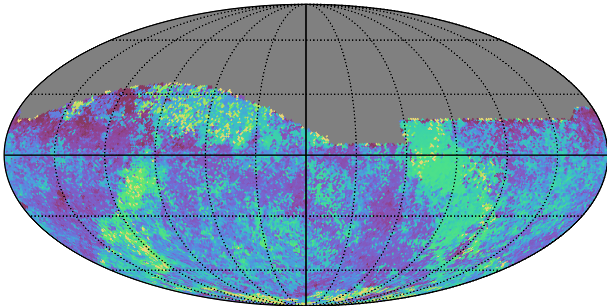
noroll_v3.4_10yrs Yr 1 all bands: Median skyBrightness
