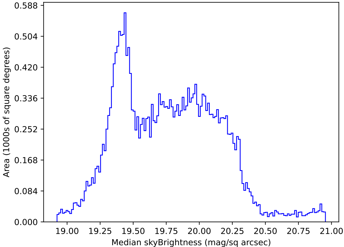
noroll_v3.4_10yrs Yr 1 all bands: Median skyBrightness
