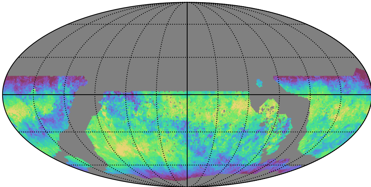
noroll_v3.4_10yrs WFD z band: Median skyBrightness
