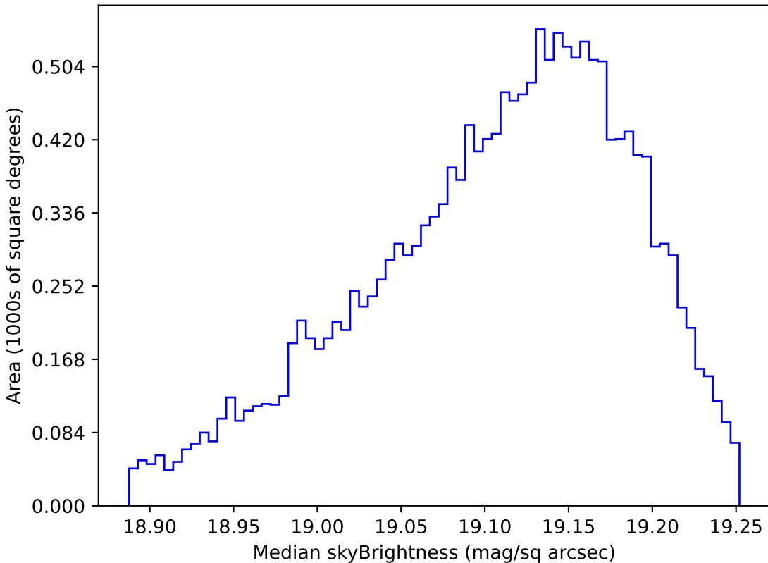
noroll_v3.4_10yrs WFD z band: Median skyBrightness
