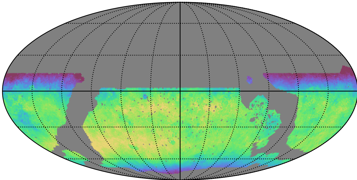
noroll_v3.4_10yrs WFD y band: Median skyBrightness
