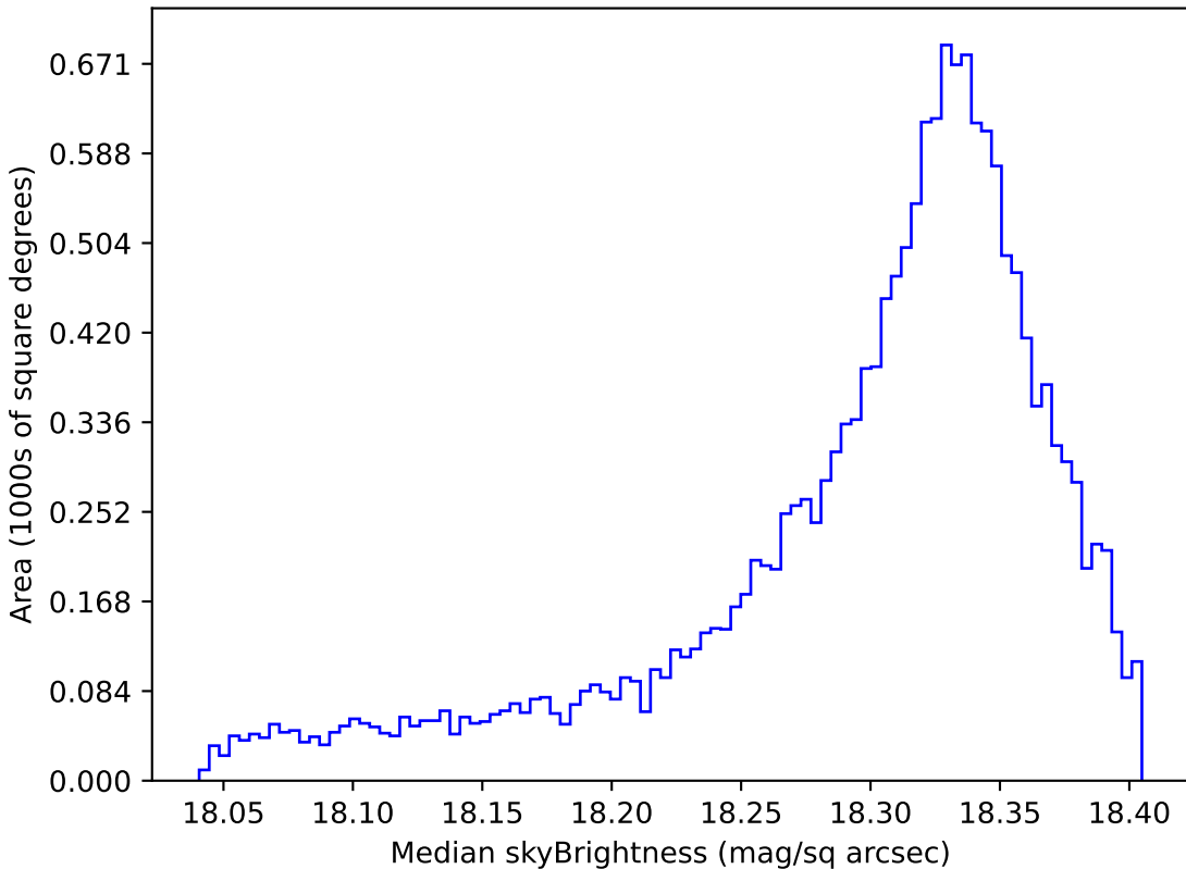
noroll_v3.4_10yrs WFD y band: Median skyBrightness
