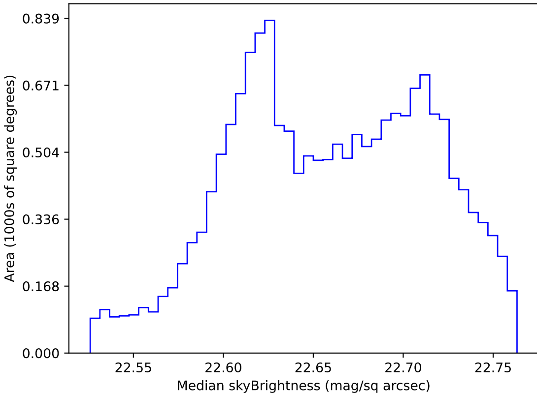
noroll_v3.4_10yrs WFD u band: Median skyBrightness
