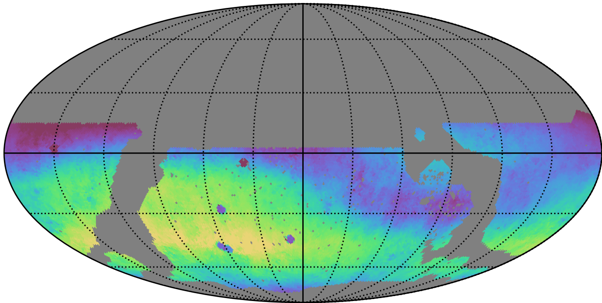
noroll_v3.4_10yrs WFD r band: Median skyBrightness
