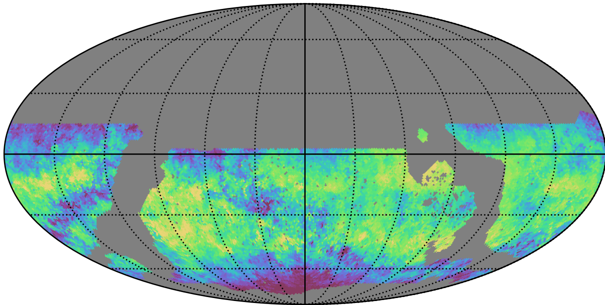
noroll_v3.4_10yrs WFD i band: Median skyBrightness
