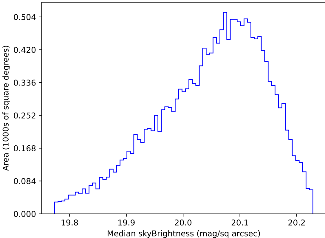
noroll_v3.4_10yrs WFD i band: Median skyBrightness
