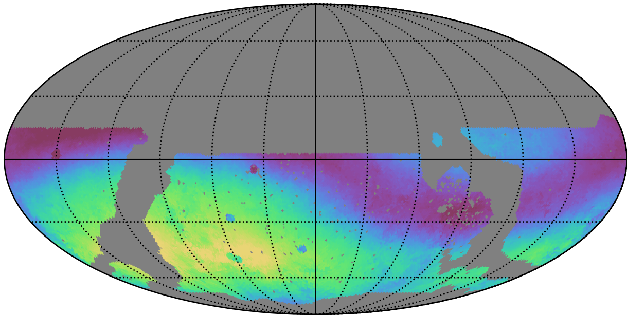
noroll_v3.4_10yrs WFD g band: Median skyBrightness
