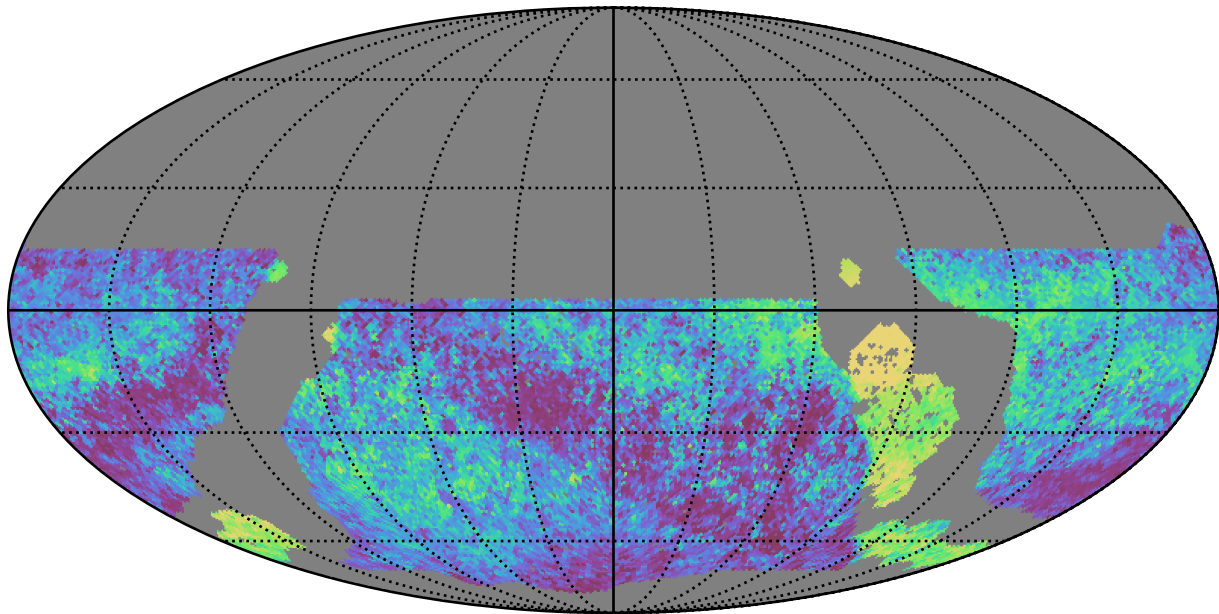
noroll_v3.4_10yrs WFD all bands: Median skyBrightness
