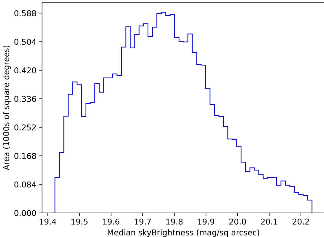
noroll_v3.4_10yrs WFD all bands: Median skyBrightness
