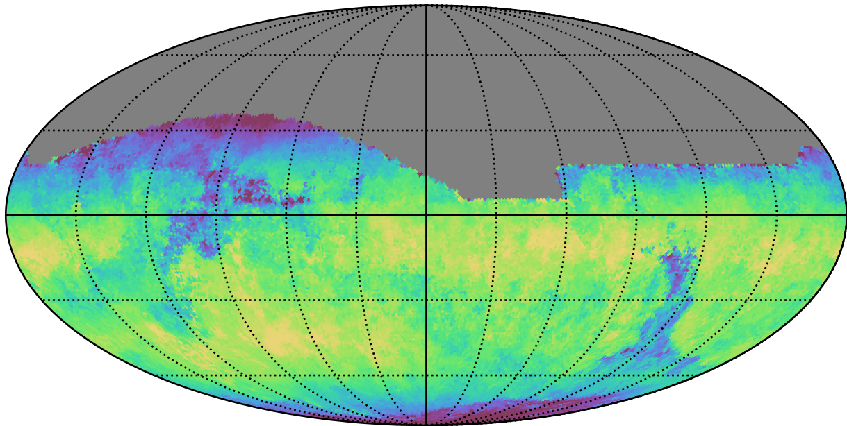
noroll_v3.4_10yrs All sky z band: Median skyBrightness
