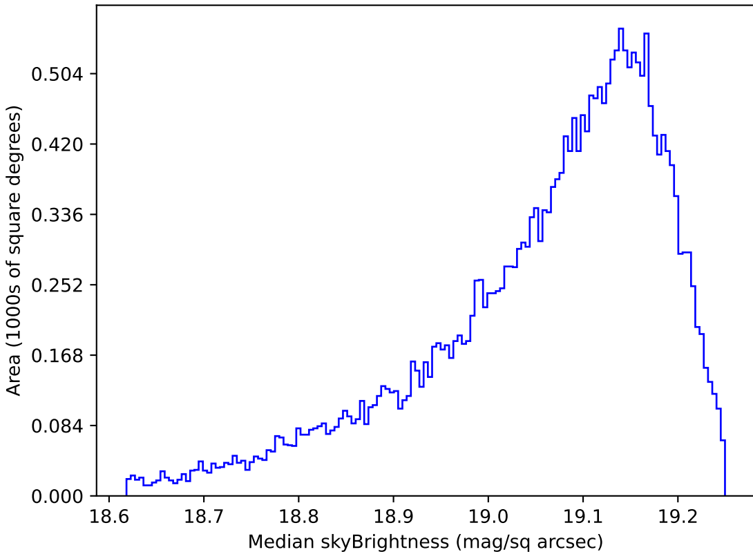
noroll_v3.4_10yrs All sky z band: Median skyBrightness
