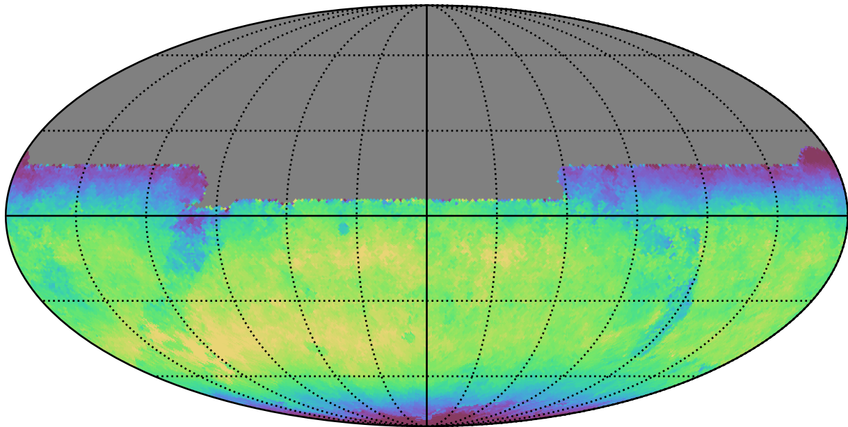
noroll_v3.4_10yrs All sky y band: Median skyBrightness
