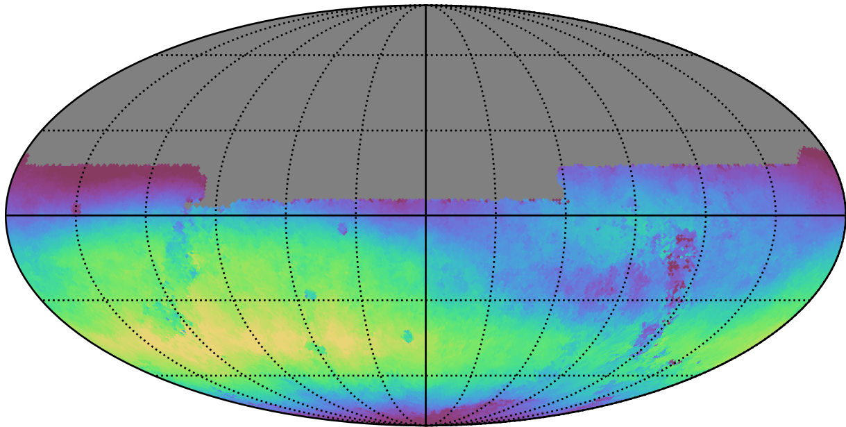
noroll_v3.4_10yrs All sky u band: Median skyBrightness
