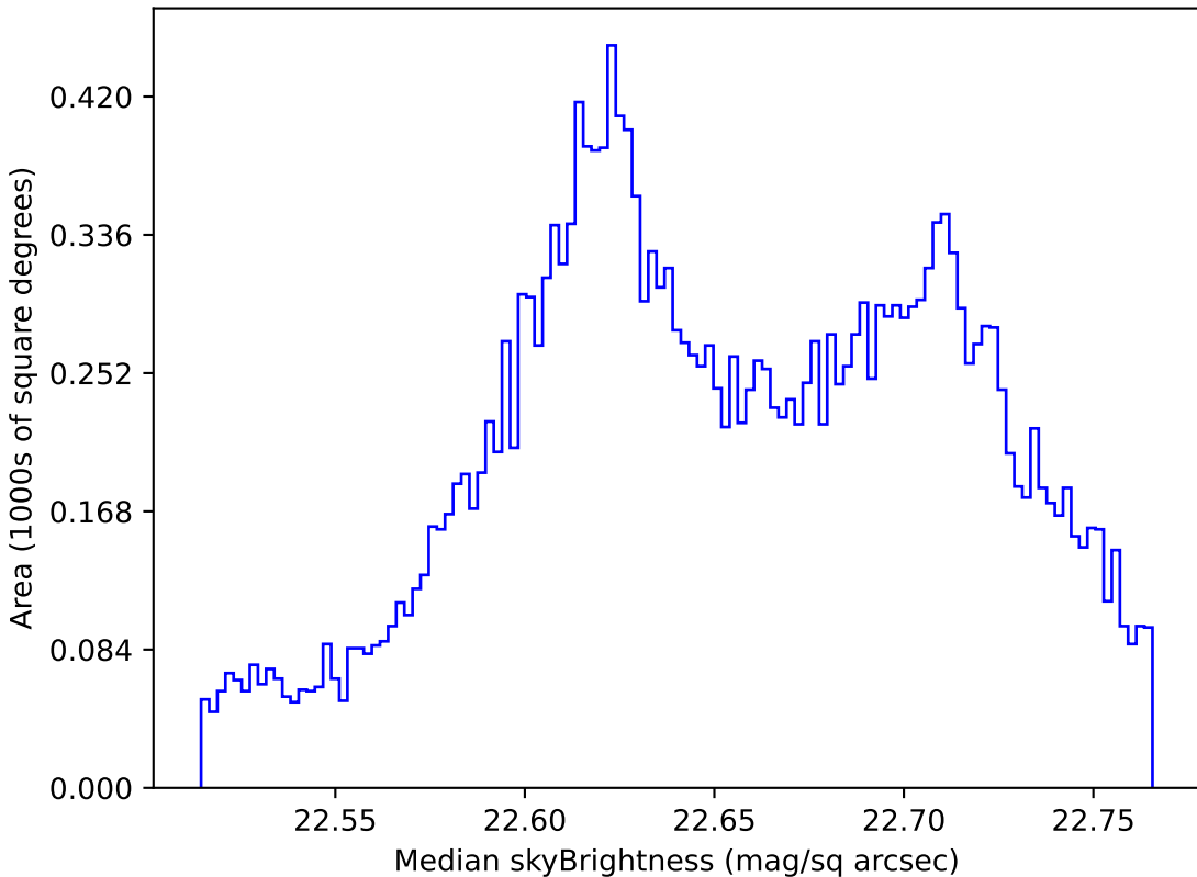
noroll_v3.4_10yrs All sky u band: Median skyBrightness
