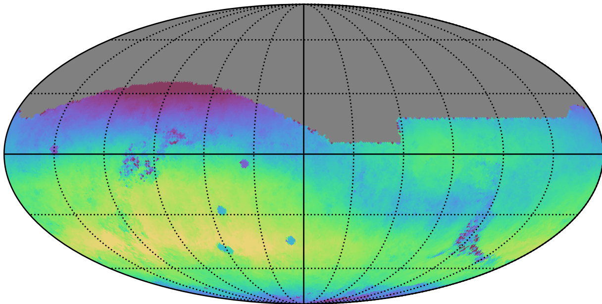
noroll_v3.4_10yrs All sky r band: Median skyBrightness
