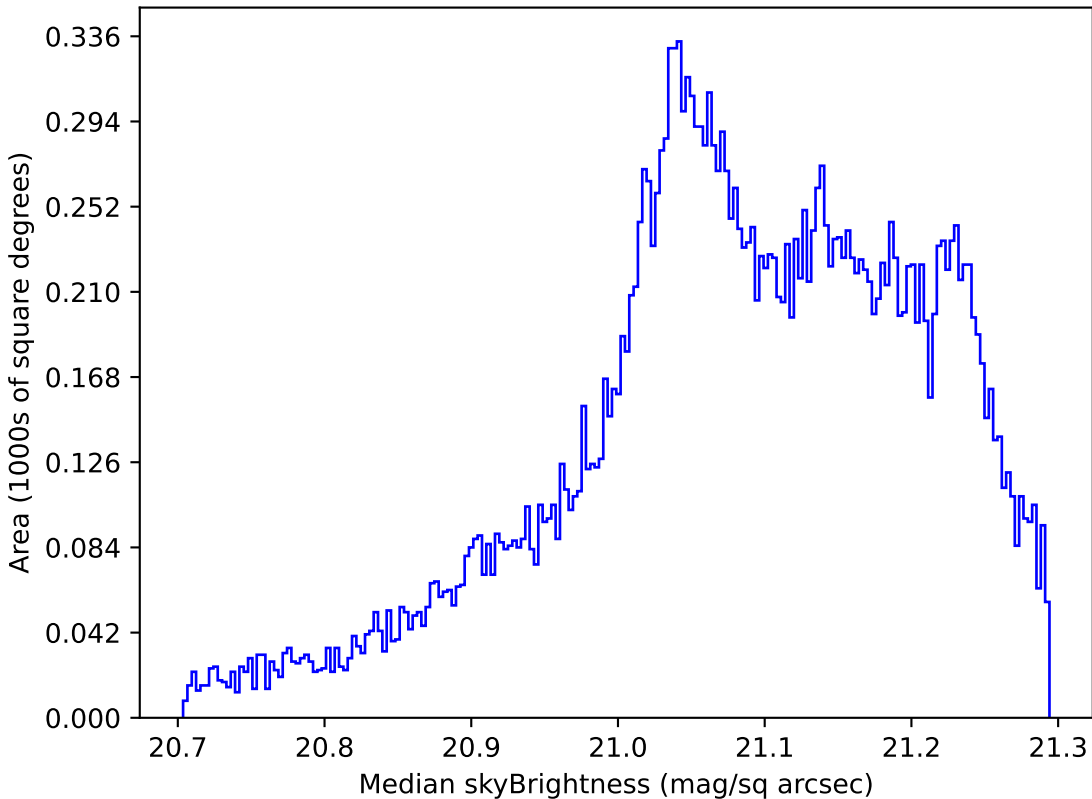
noroll_v3.4_10yrs All sky r band: Median skyBrightness
