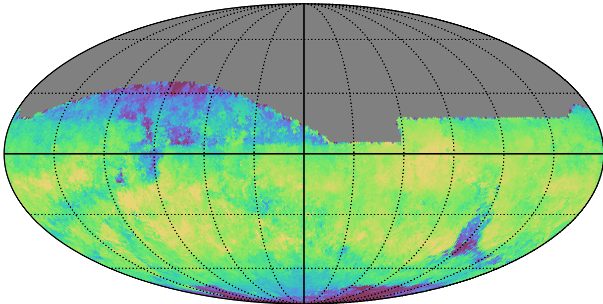
noroll_v3.4_10yrs All sky i band: Median skyBrightness
