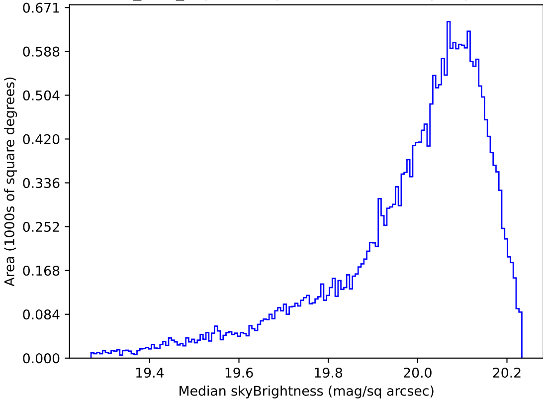
noroll_v3.4_10yrs All sky i band: Median skyBrightness
