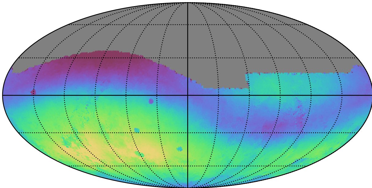
noroll_v3.4_10yrs All sky g band: Median skyBrightness
