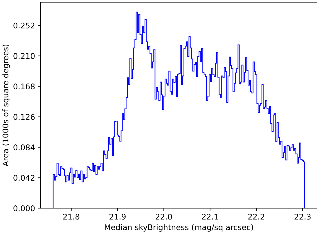
noroll_v3.4_10yrs All sky g band: Median skyBrightness
