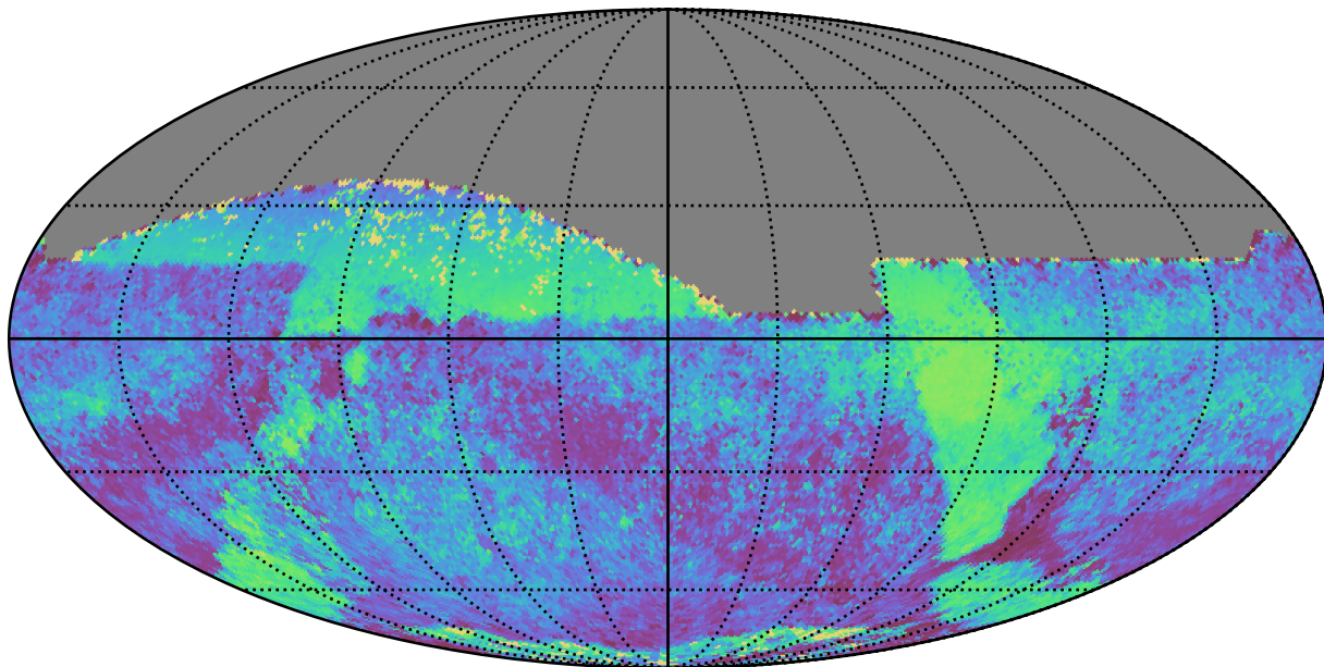
noroll_v3.4_10yrs All sky all bands: Median skyBrightness
